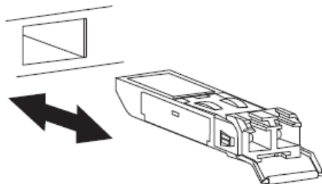
SFP Module Insertion (Bail shown in unlocked position)
